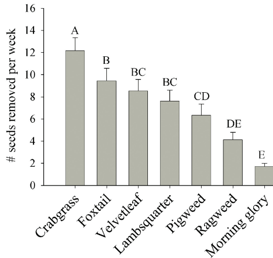
Fig. 2. Mean ± SEM preference for weed seed species by granivorous arthropods under field conditions. The average number of seeds (SEM) consumed per plot over 3 wk (n=12). Bars with different letters are significantly different ( \alpha=0.05 , LSD test).
